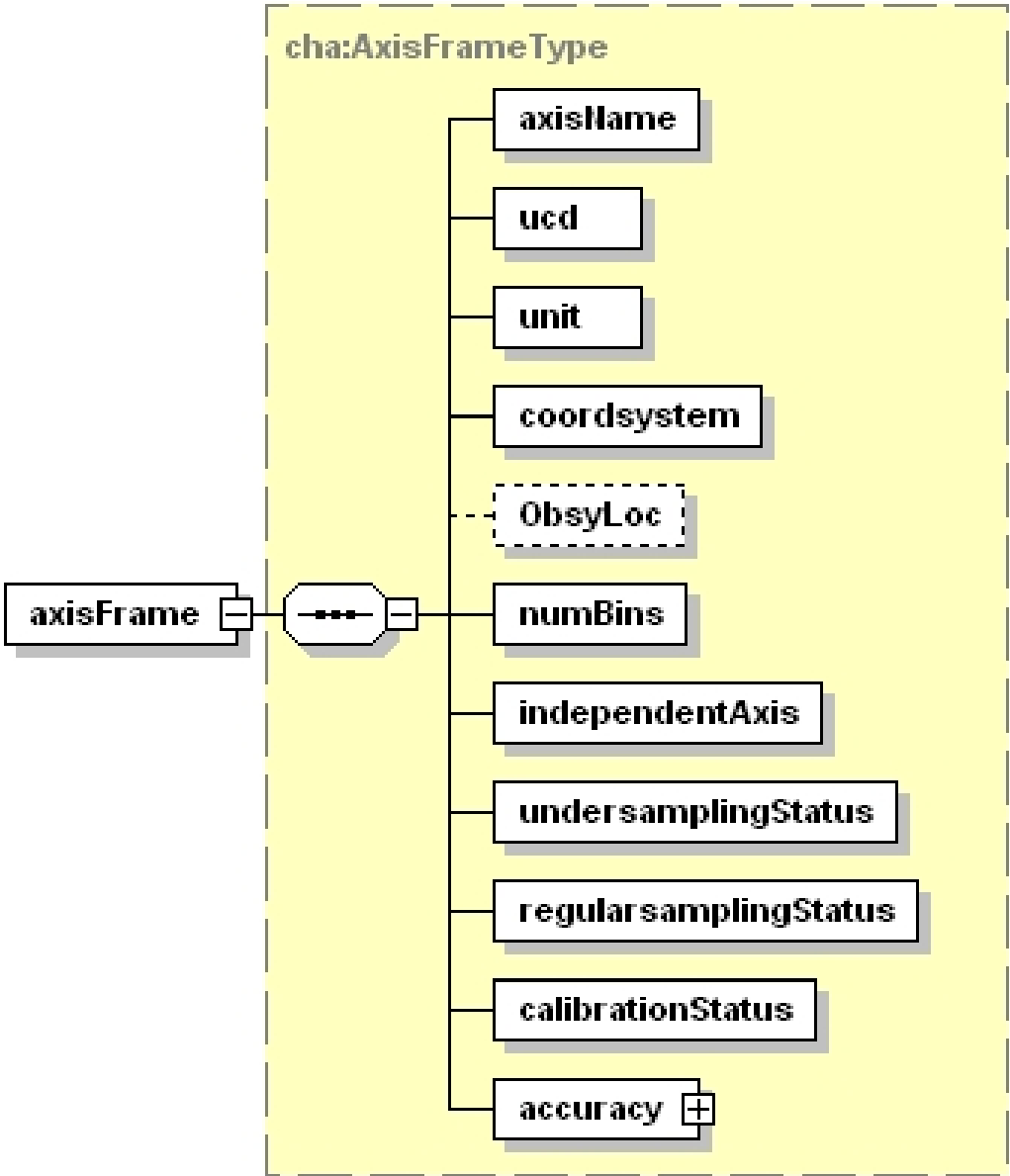
Figure 7: The coordSystem and ObsyLoc items are STC elements. Other elements are derived from the UML class AxisFrame .
