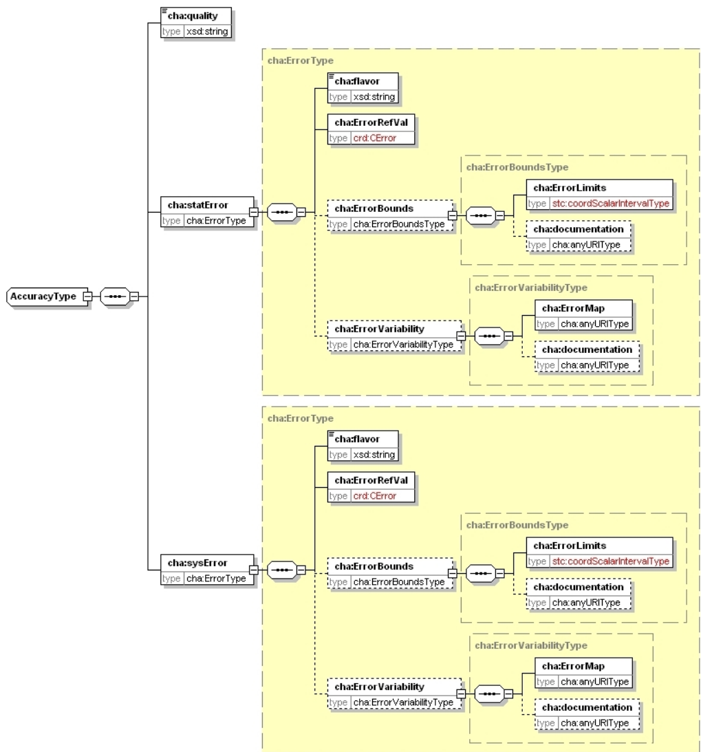
Figure 12: This graphical view was generated with XMLSPY from the accuracy element of the schema.
