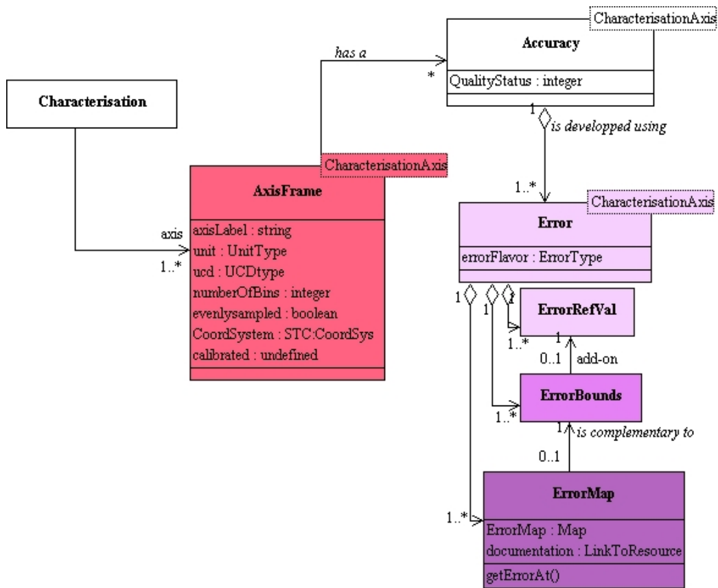
Figure 5: This class diagram illustrates the AxisFrame class and its relationship with the Accuracy class, which encompasses various classes of errors such as systematic or statistical.
