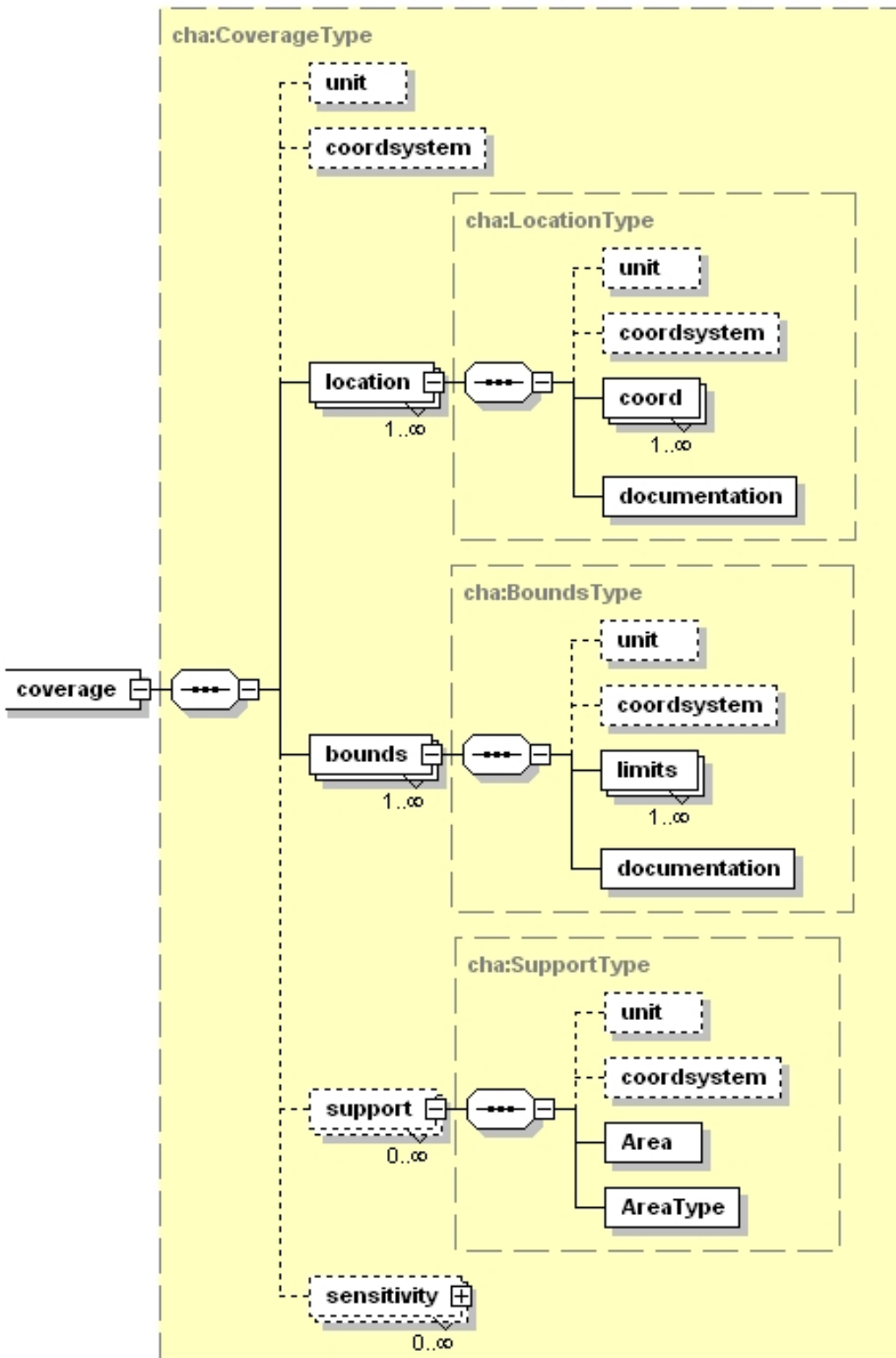
Figure 8: The coordsystem and unit items can be factorised at the top of the Coverage structure, but may be redefined at each level when necessary. Bounds are expressed using a limits element which is developed on a general bounding box type: CharCoordArea. AreaType is a string describing the kind of region used: Circle, Polygon etc.
