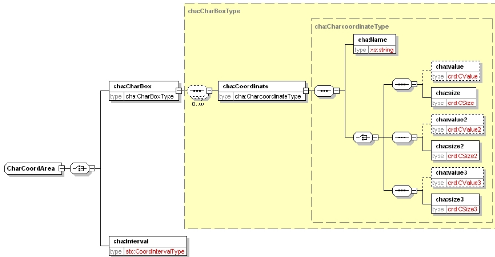
Figure 9: Representing limits: The two expressions allowed for a bounding box are expressed using either a STC:CoordInterval directly or build on another type: CharBox representing a generic centered box in N-dimensions.
