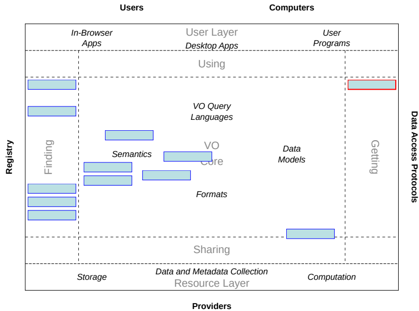
Figure 1: Architecture diagram for Simple Cone Search
