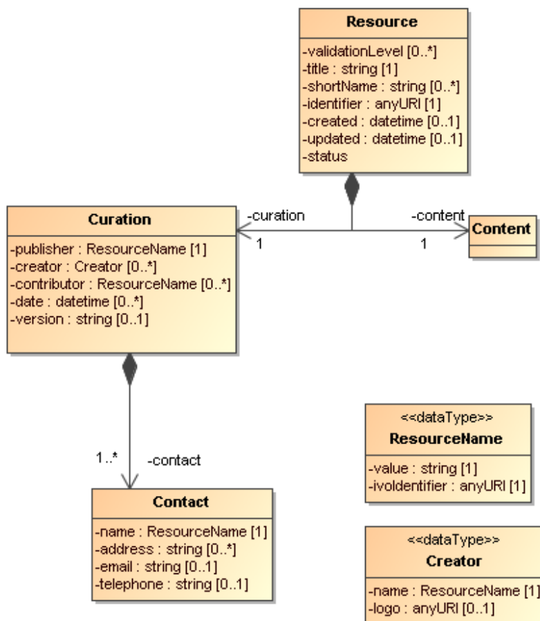
Figure 11 UML rendering of the Resource complexType from [14].
