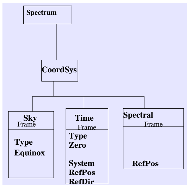
Figure 4: Diagram for CoordSys object
