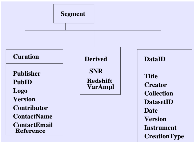
Figure 5: Diagram for Curation, DataID, Derived objects
