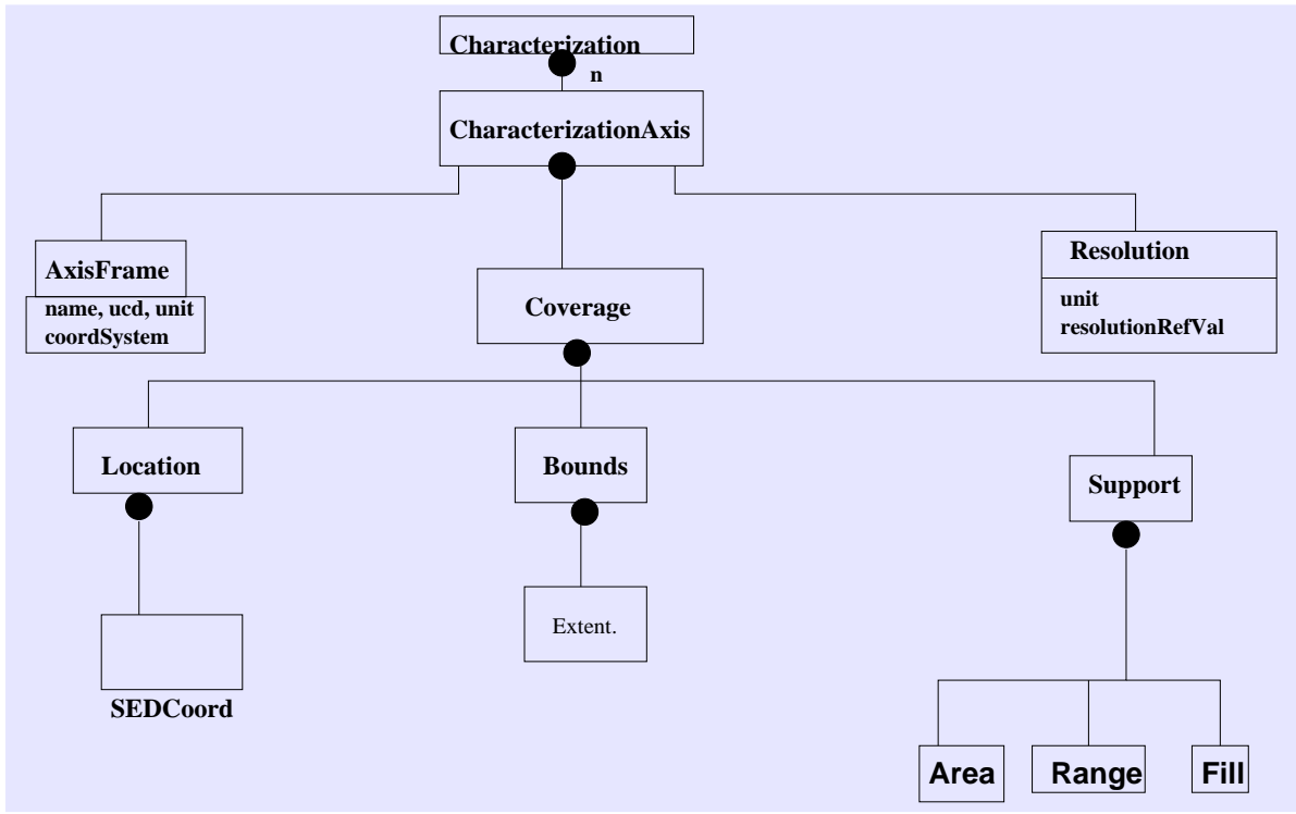
Figure 3: Diagram for Coverage object
